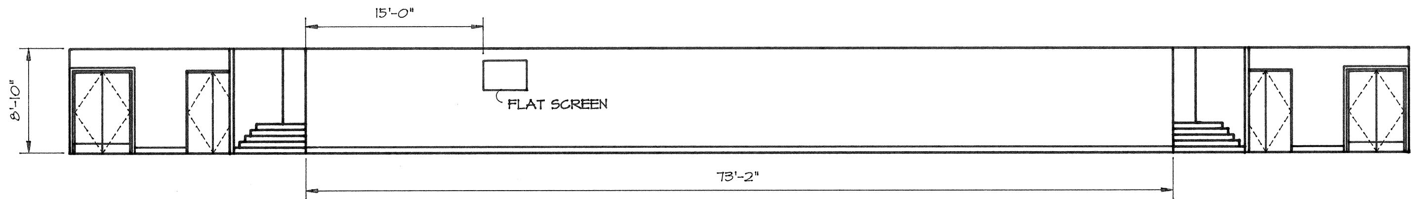
ELEVATION 'A'
